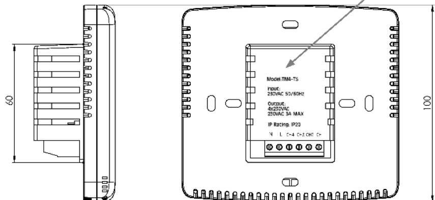
Wiring Detail
