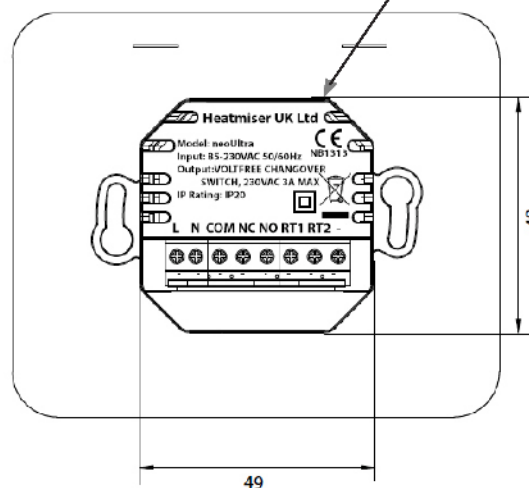
Wiring Detail
