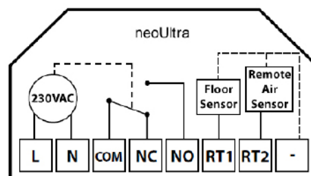
Wiring Detail
