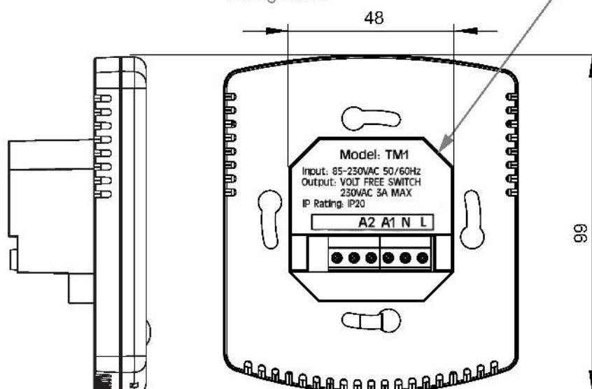
Wiring Detail
