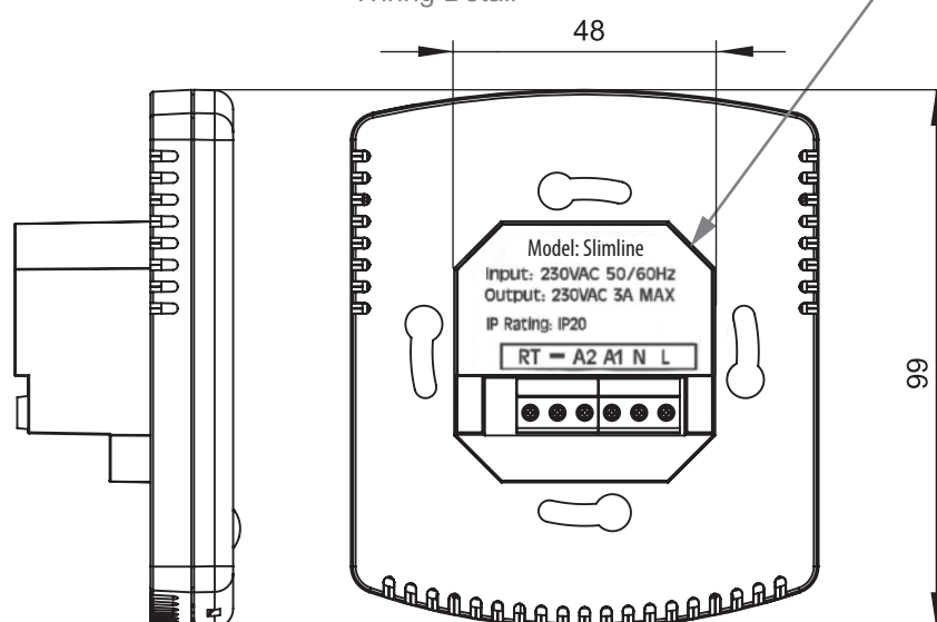
Wiring Detail
